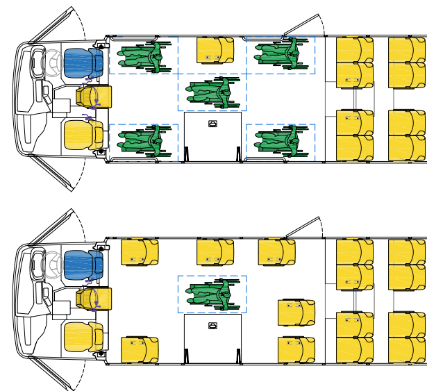
輪椅復康車 - 輪椅佈局 Electric Rehabilitation Bus - Wheelchair Layout options
